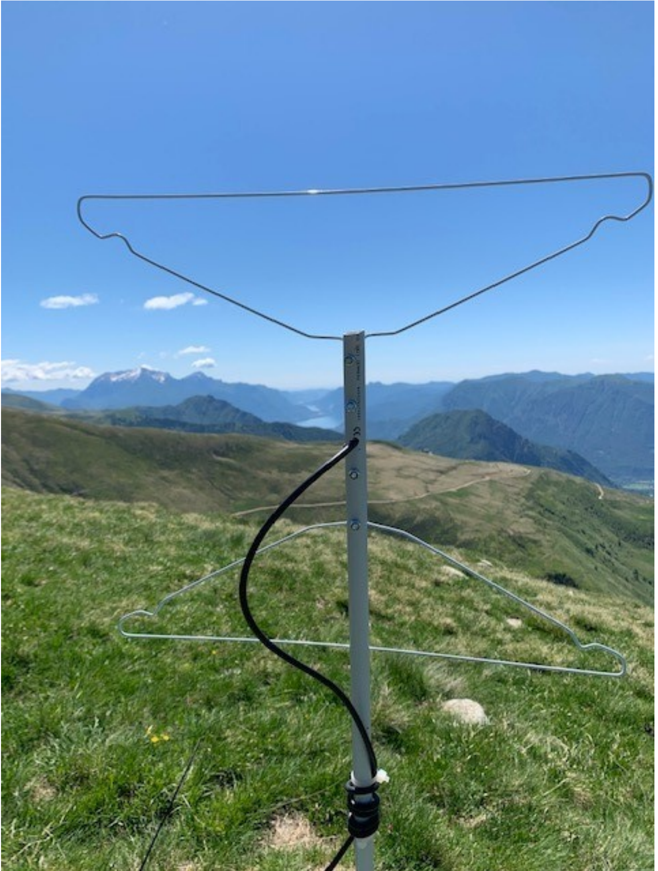
mega antenna
